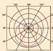
BELTR LED TUBE 1x120
