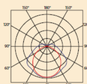
BELTR LED TUBE 2x120
