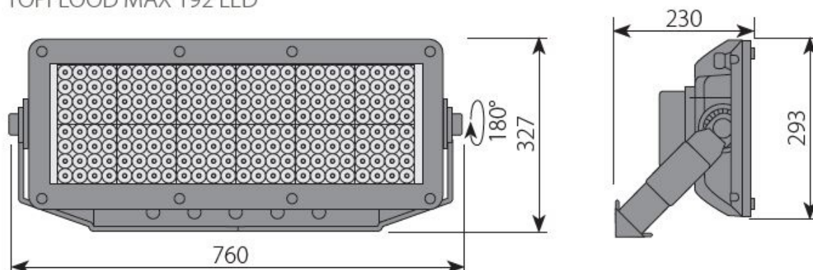
TOPFLOOD MAX 192 LED
